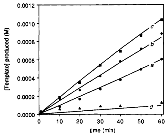
Figure 6. Experimental (points) and calculated (lines) generation of template 11a or 11b as a function of time. All reactions were performed with initial concentrations [9] = [10d or 10h] = 0.0082 M in CHCl 3 . (a) Reaction of 9 and 10d . (b) Reaction of 9 and 10d with 0.20 equiv of 11a added as autocatalyst. (c) Reaction of 9 and 10d with 0.50 equiv of 11a added as autocatalyst. (d) Reaction of 9 and the N-methylated 10h .
